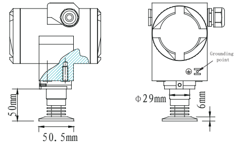
Figure 6-2 Tri-Clamp
