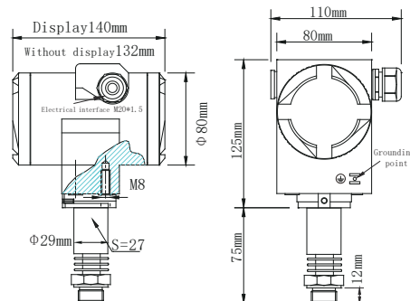
Figure 6-1 Threaded connection
